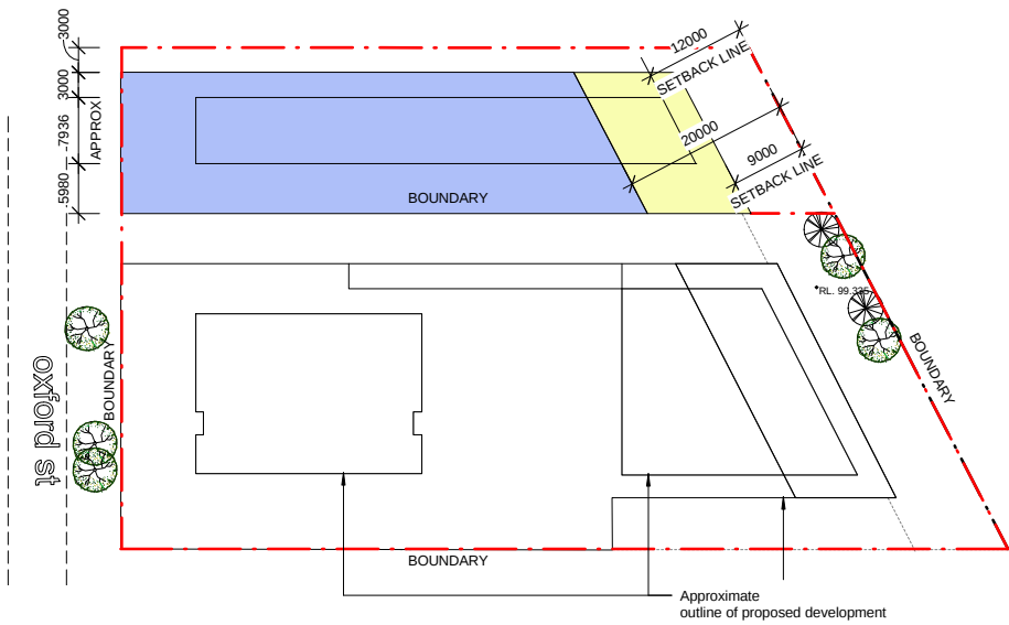
PODIUM FLOOR PLATE
